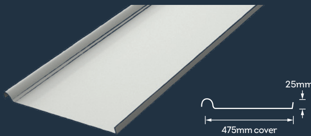
Neo Roman™ 475mm Single Rib
