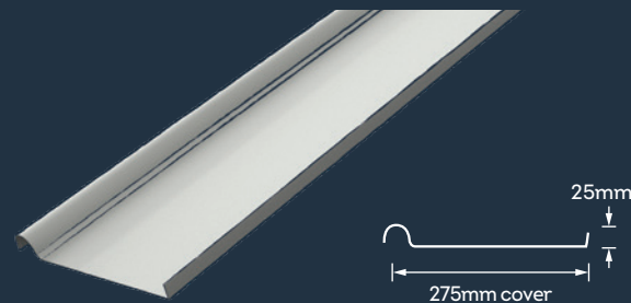
Neo Roman™ 275mm Single Rib
